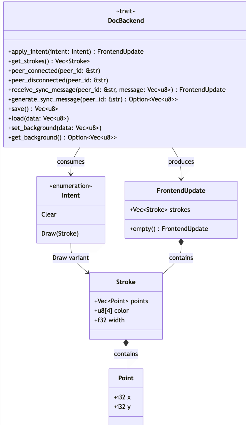
Figure 2.4: Backend Interface
